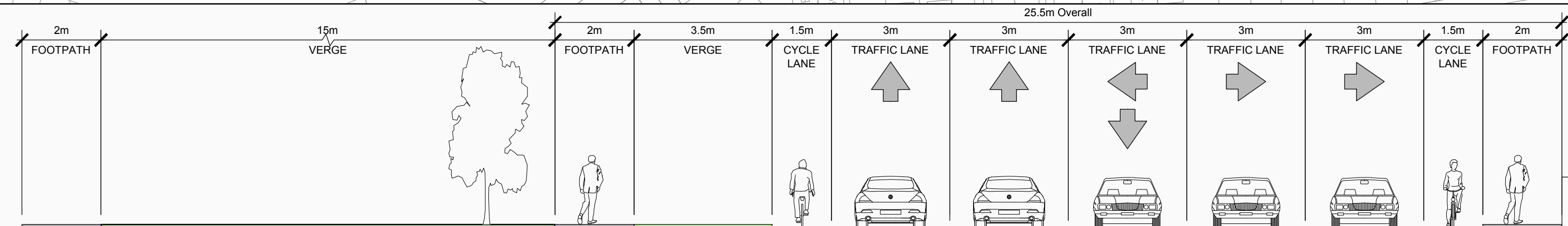
EXISTING SECTION A-A SCALE 1:100 @ A1
