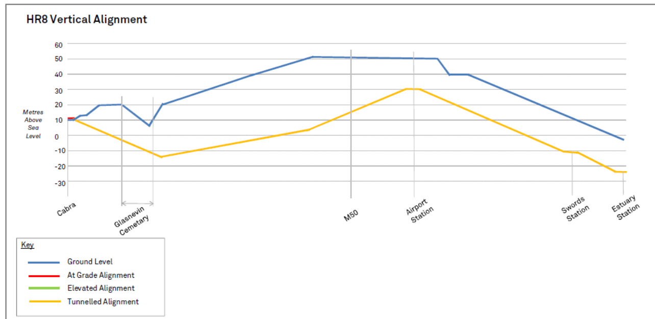
Figure 7.14: Vertical Alignment
