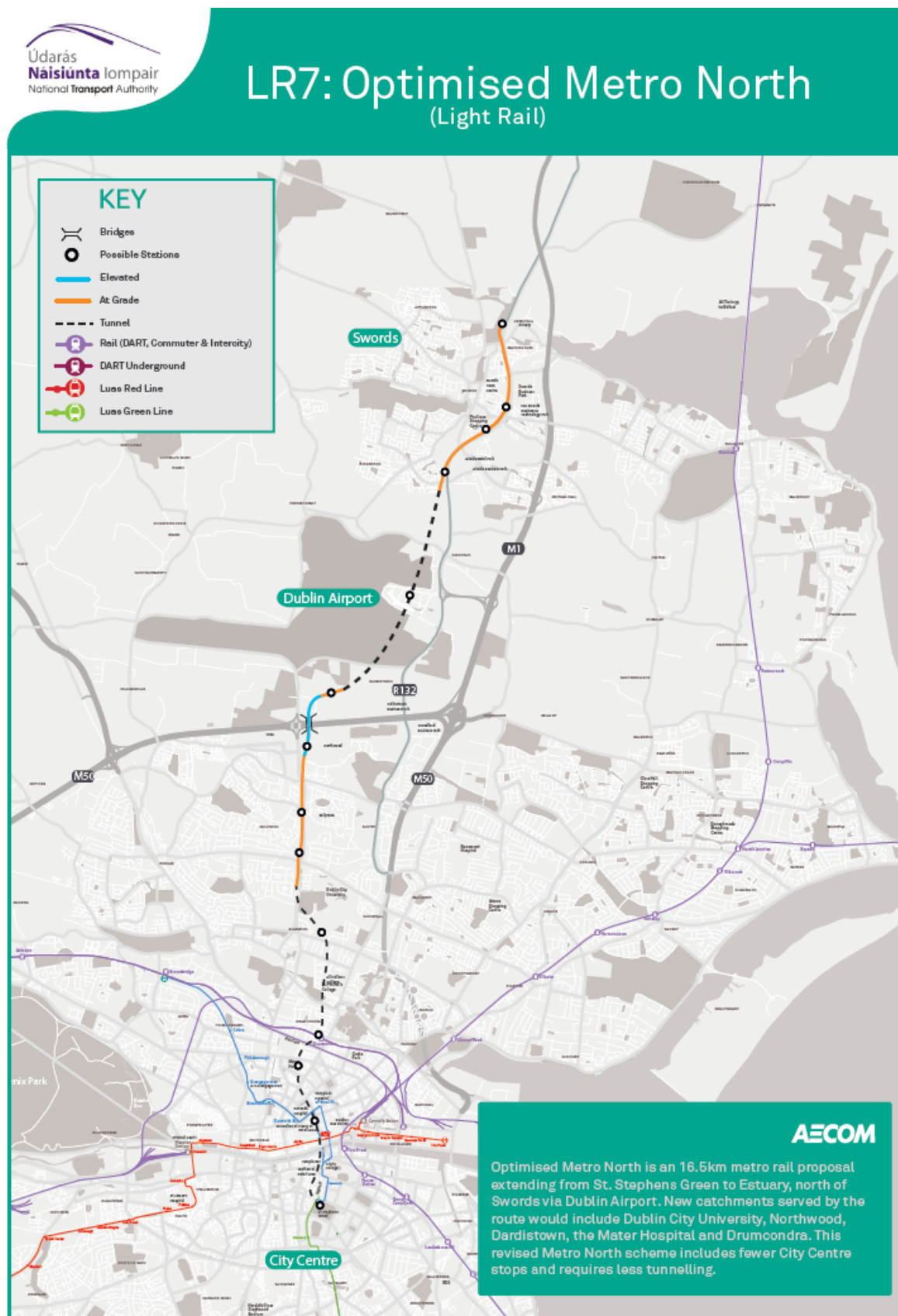
Figure 8.17: Proposed Alignment for LR7
