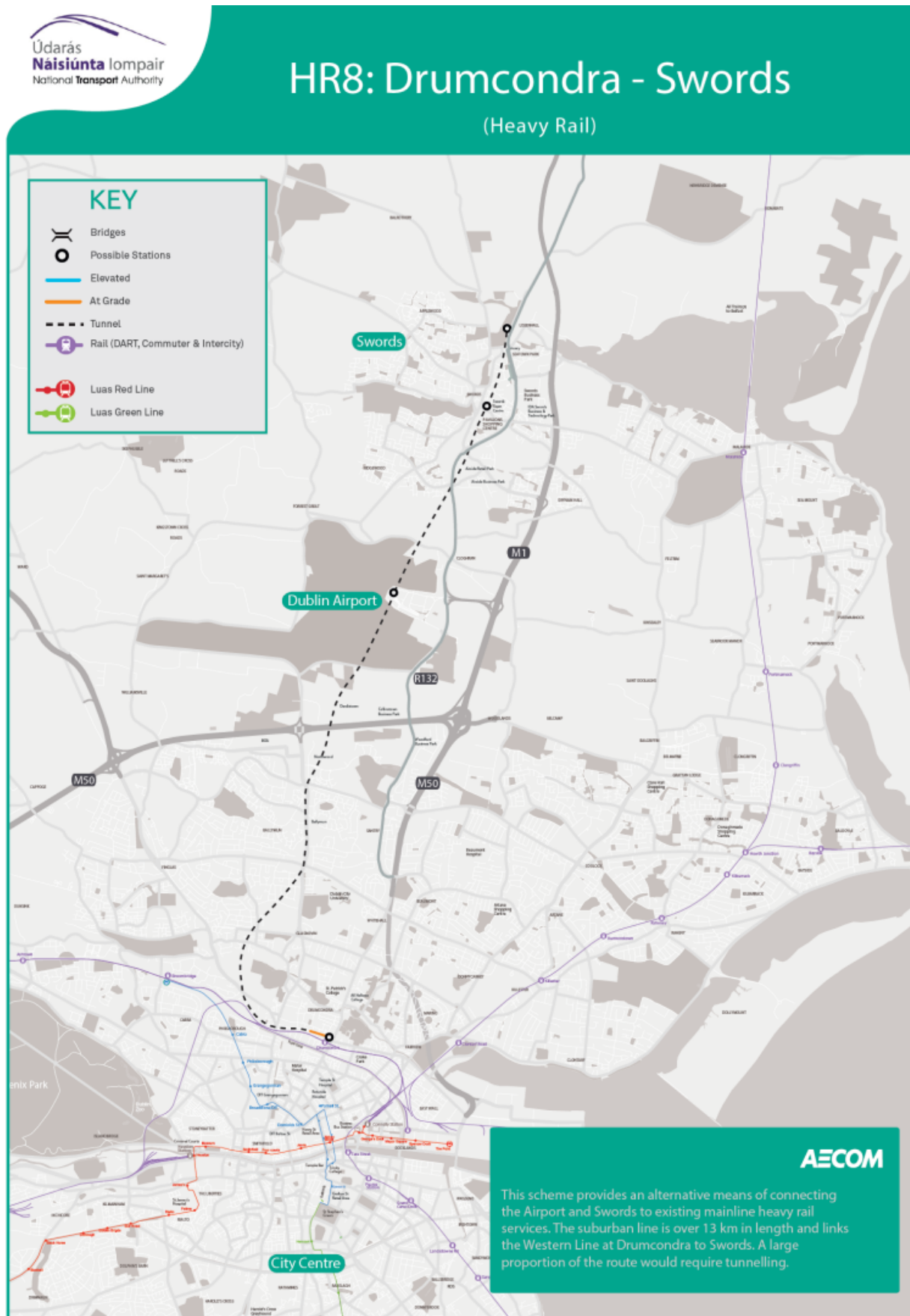
Figure 7.15: Proposed Alignment for HR
