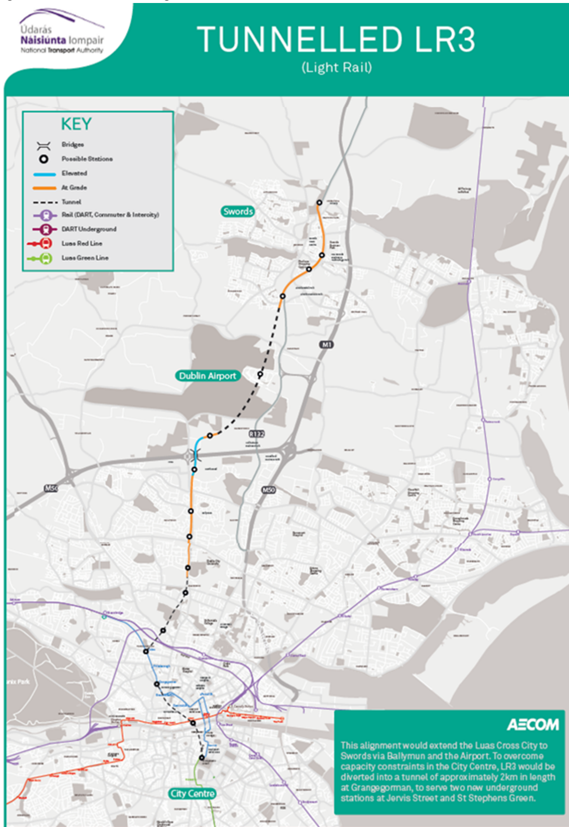
Figure 8.12: Tunnelled LR3 alignment
