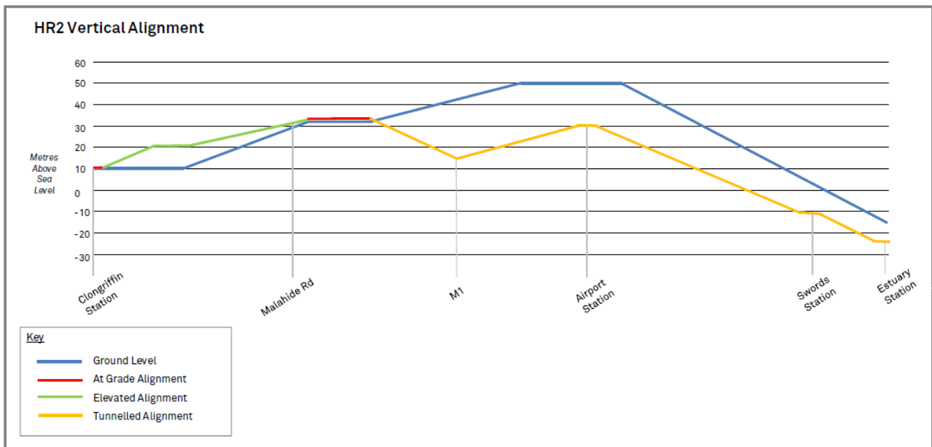
Figure 7.5: Indicative vertical alignment for HR2
