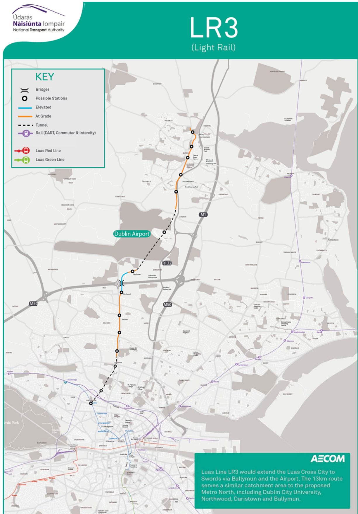
Figure 8.2: Proposed Alignment for LR3
