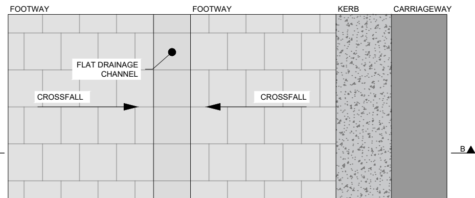
TYPICAL FLAT DRAINAGE CHANNEL IN FOOTWAY
