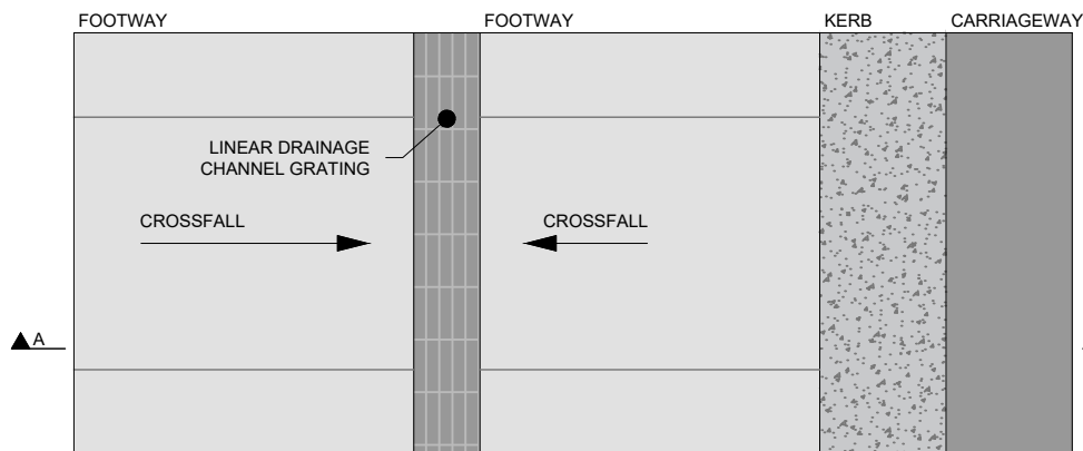
TYPICAL LINEAR DRAINAGE CHANNEL IN FOOTWAY
