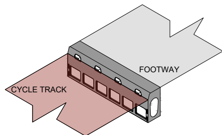
DRAINAGE KERB (ISOMETRIC)
