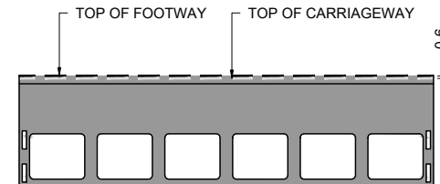
TYPICAL DRAINAGE KERB AT PEDESTRIAN CROSSING
