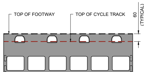
TYPICAL DRAINAGE KERB ADJACENT TO CYCLE TRACK
